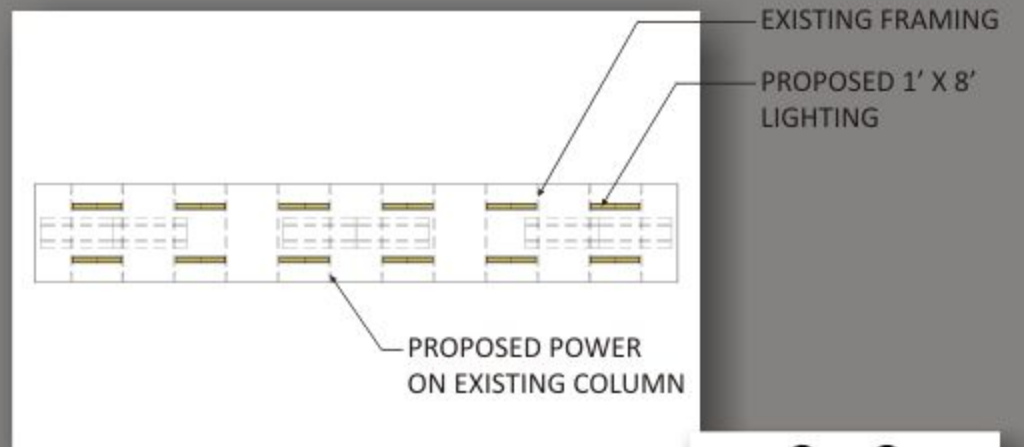
PROPOSED LIGHTING PLAN AT SHADE STRUCTURE
