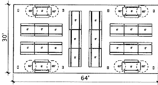
PICNIC SEATING FOR 196
