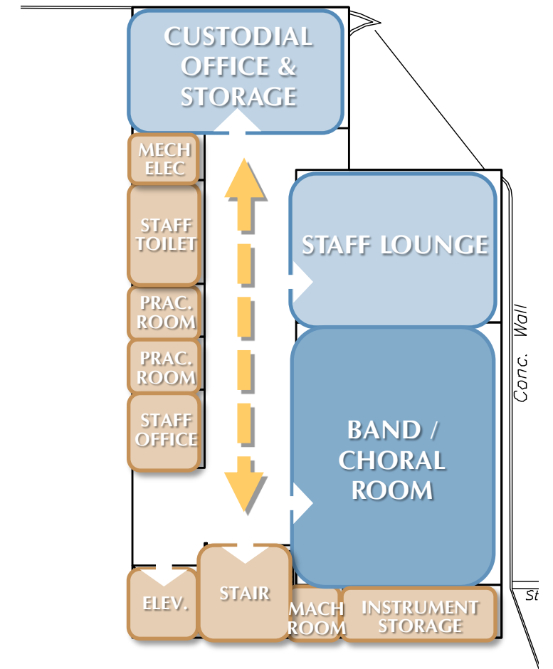
BLDG. C LOWER LEVEL
